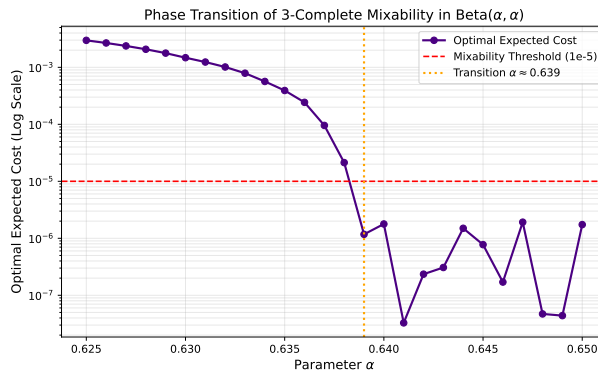
Figure 10: Optimal cost for symmetric Beta( \alpha, \alpha ), \alpha \in [0.625, 0.65] , N = 45 . The transition occurs between \alpha = 0.638 and \alpha = 0.639 .
